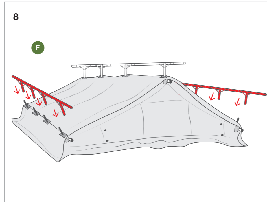
Slot a shade net frame onto the joint pins along the each side.
