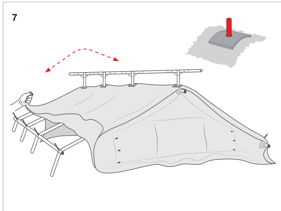
Spread out the outer tent and secure by inserting side joint pins through the eyelets. Ensure that the ends of the "A" poles are exposed
