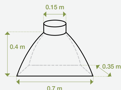
Heat-resistant sleeve
