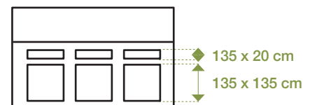
Side view (Window and ventilation)
