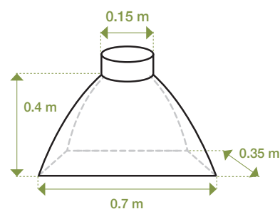
Heat-resistant sleeve
