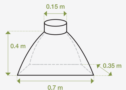
Heat-resistant sleeve
