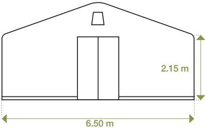
Front/Side View
