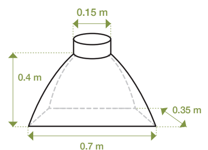
Heat-resistant sleeve
